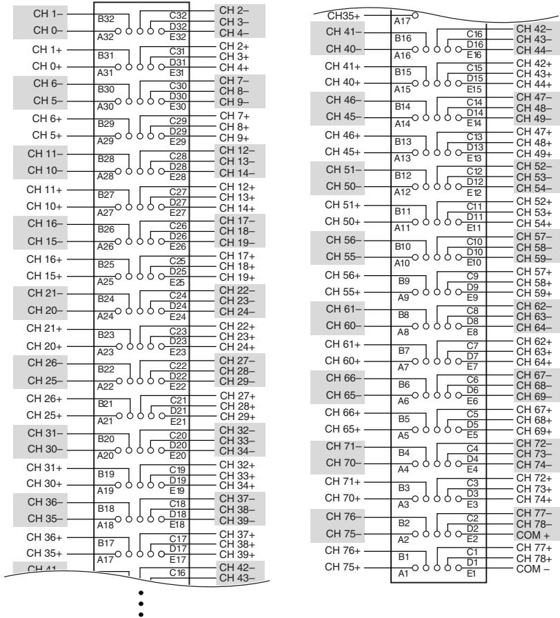
Figure 3. NI 2526 2-Wire Pinout
